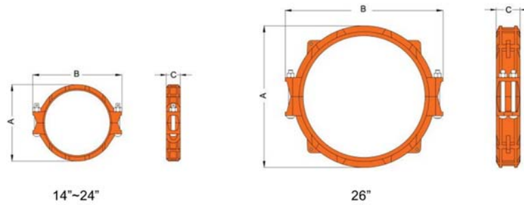
Model 7707N Heavy Duty Flexible Coupling
