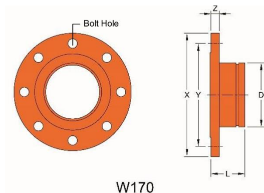
Model W170 Flange Adapter ANSI Class 125/150
