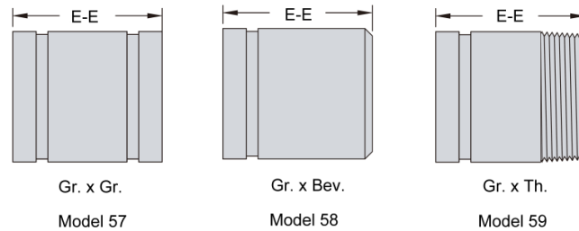
Model 57 / 58 / 59 Nipples
