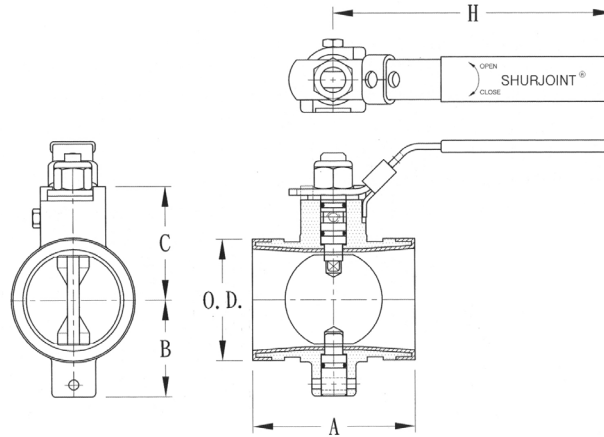
Model SJ-200 Low-Profile Butterfly Valve
