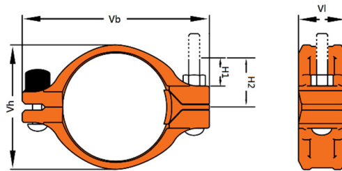
M07 Quick Install Coupling
